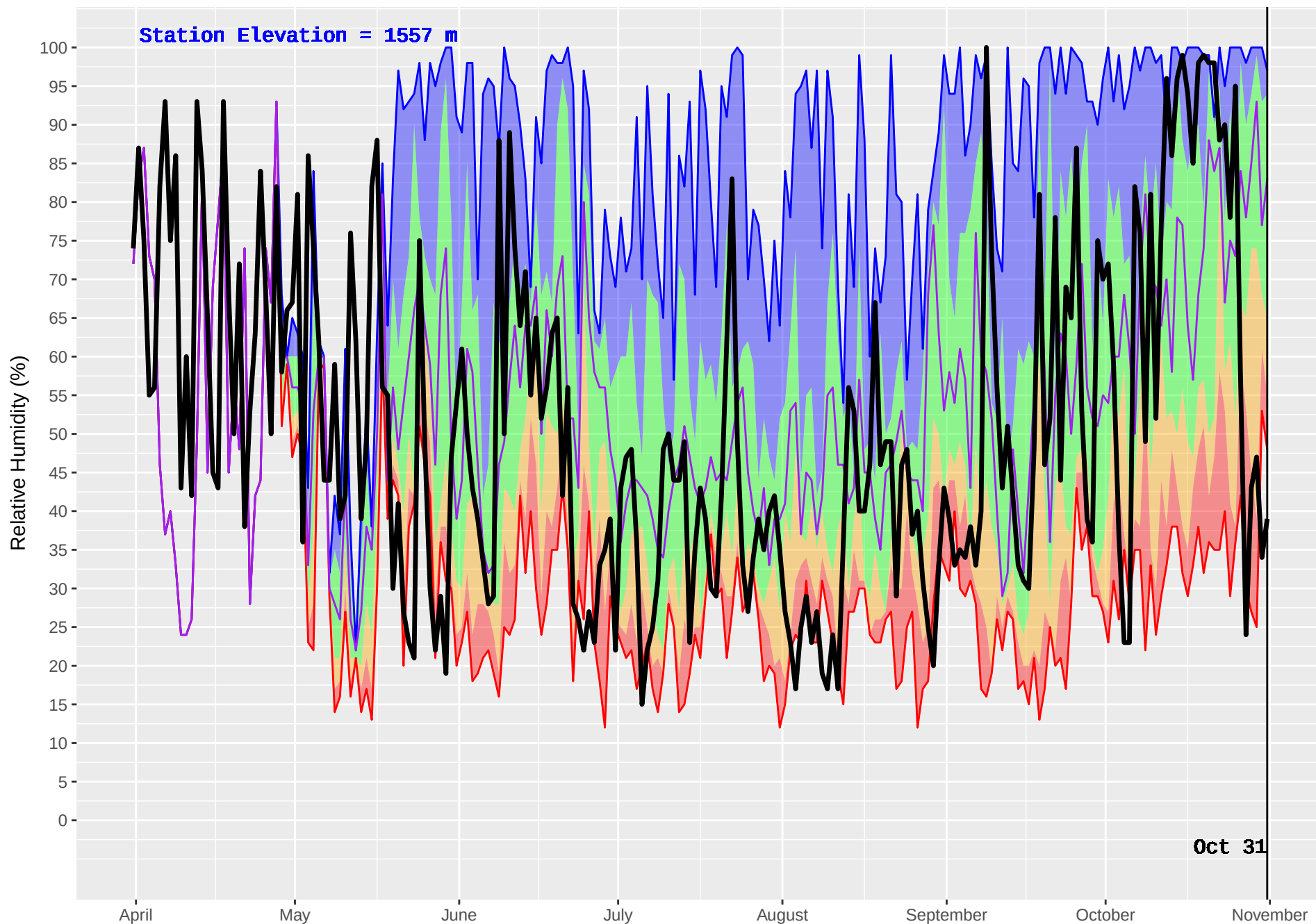
SKOONKA (1024) : Historical (2008–2016) and Current (2017) Noon Relative Humidity
