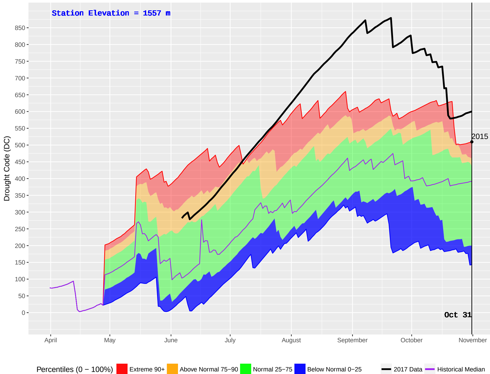
SKOONKA (1024) : Historical (2008–2016) and Current (2017) Noon Drought Code (DC)
