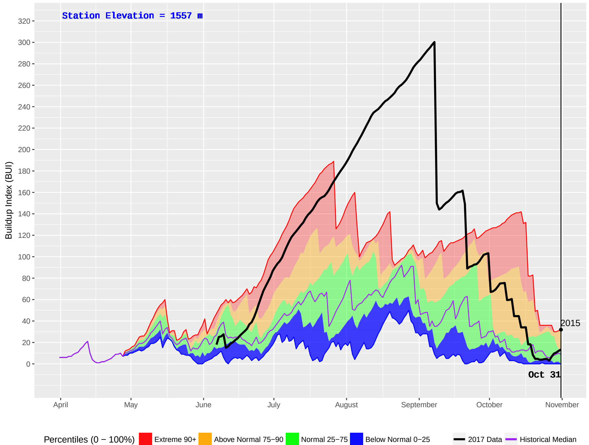
SKOONKA (1024) : Historical (2008–2016) and Current (2017) Noon Buildup Index (BUI)
